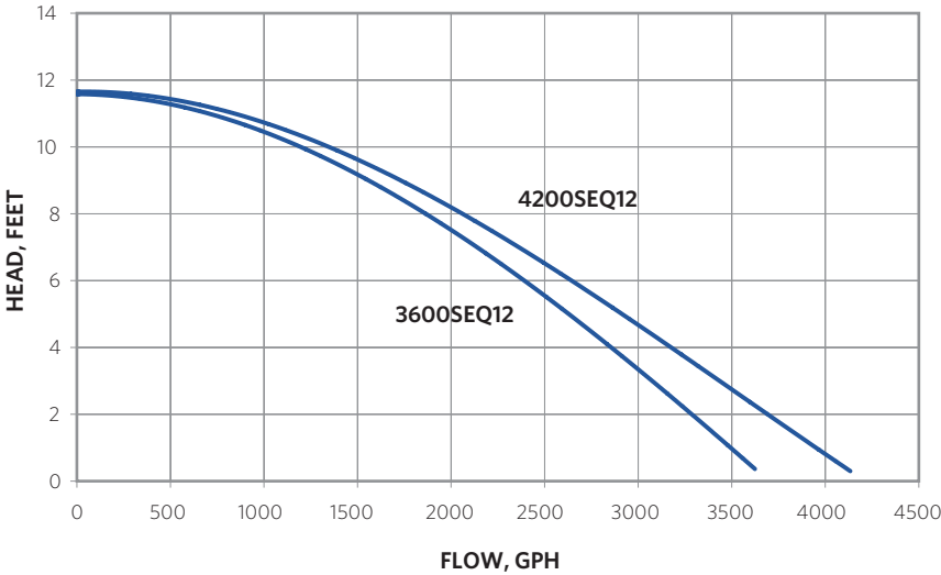
750 FAMILY PERFORMANCE CURVES
