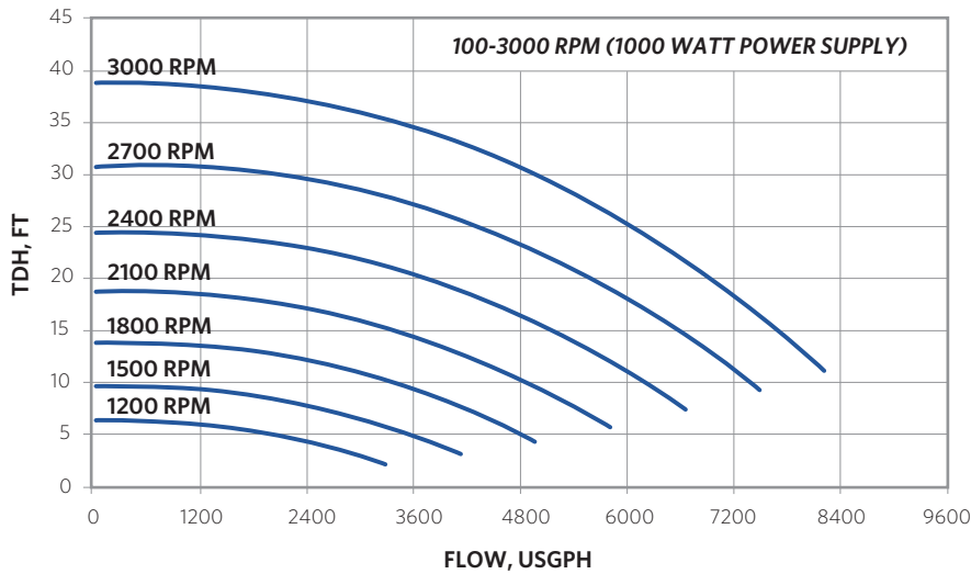
COLOSSUS 750 DC PLUS FAMILY PERFORMANCE CURVES
