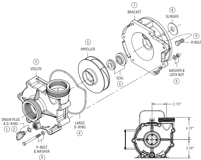
Pump end and motor illustrations are for reference only.
