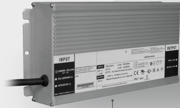
100-240V POWER SUPPLY
