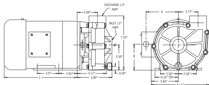
ADVANCE 3000 PUMP SCHEMATIC
