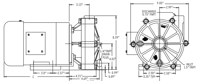
ADVANCE 1000 PUMP SCHEMATIC
