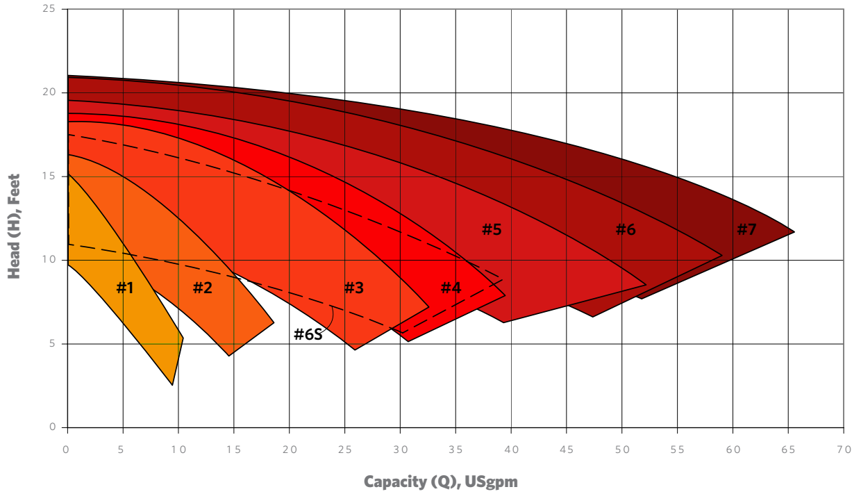
1725 rpm
